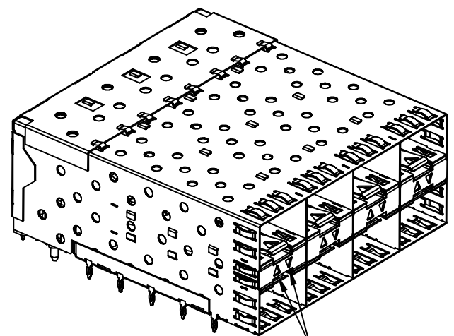
With Inner Light Pipe
