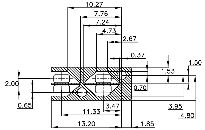
Detail-Lightpipe Location and Other Zones Scale 2:1
