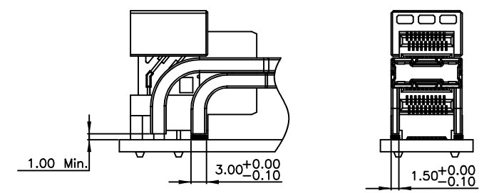
LED Clearance Requirements
