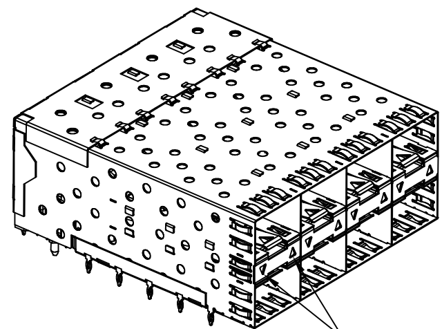
With Outer Light Pipe
