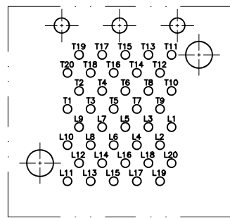
Conncton Pinout Detail Component Side of Board
