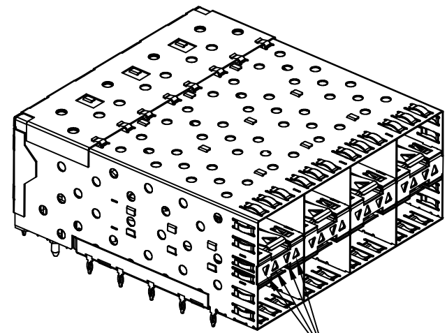
With Inner/Outer Light Pipe
