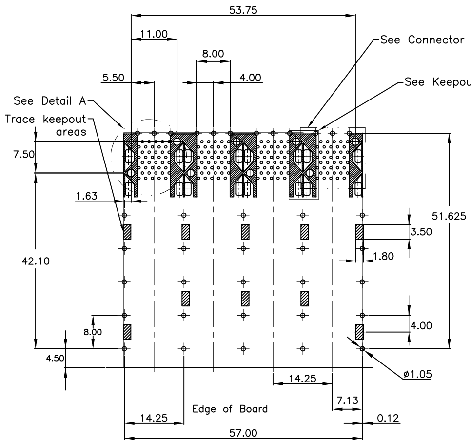
Recommended P.C. Board Layout (Component Side) P.C. Board Tolerance \pm 0.05
