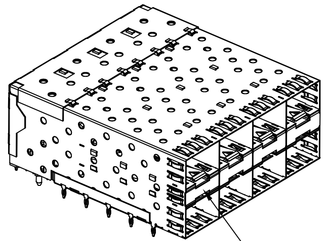
Without Light Pipe
