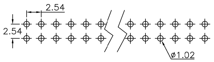
P.C. Board Layout
